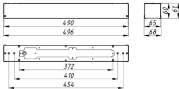
a) Trade Linear 490x65x60
