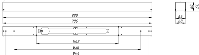
b) Trade Linear 980x65x60
